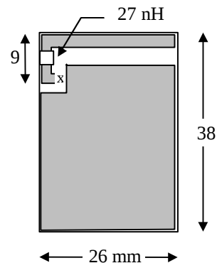
Short Stub: 916.5 MHz
