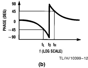
FIGURE 4. 2nd-Order Notch Response
