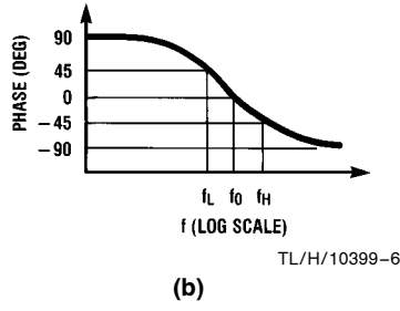
FIGURE 1. 2nd-Order Bandpass Response
