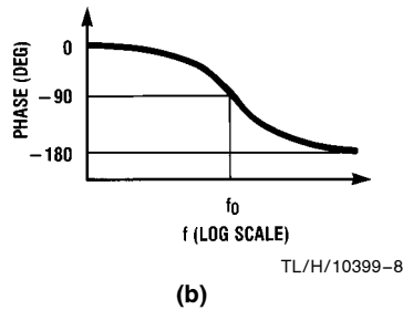
FIGURE 2. 2nd-Order Low-Pass Response
