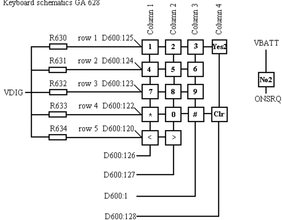
Keyboard schematics GA 628
